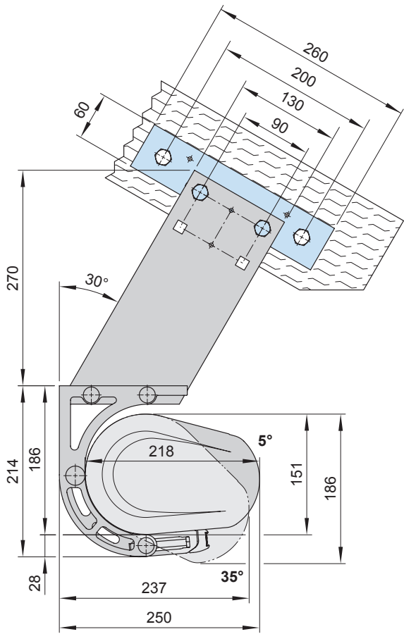
With eaves fixture bracket 270 mm (77940.)
