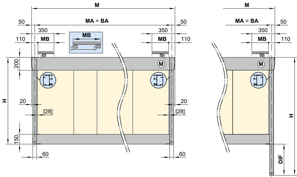
Guide track variant, asymmetrical lengths
