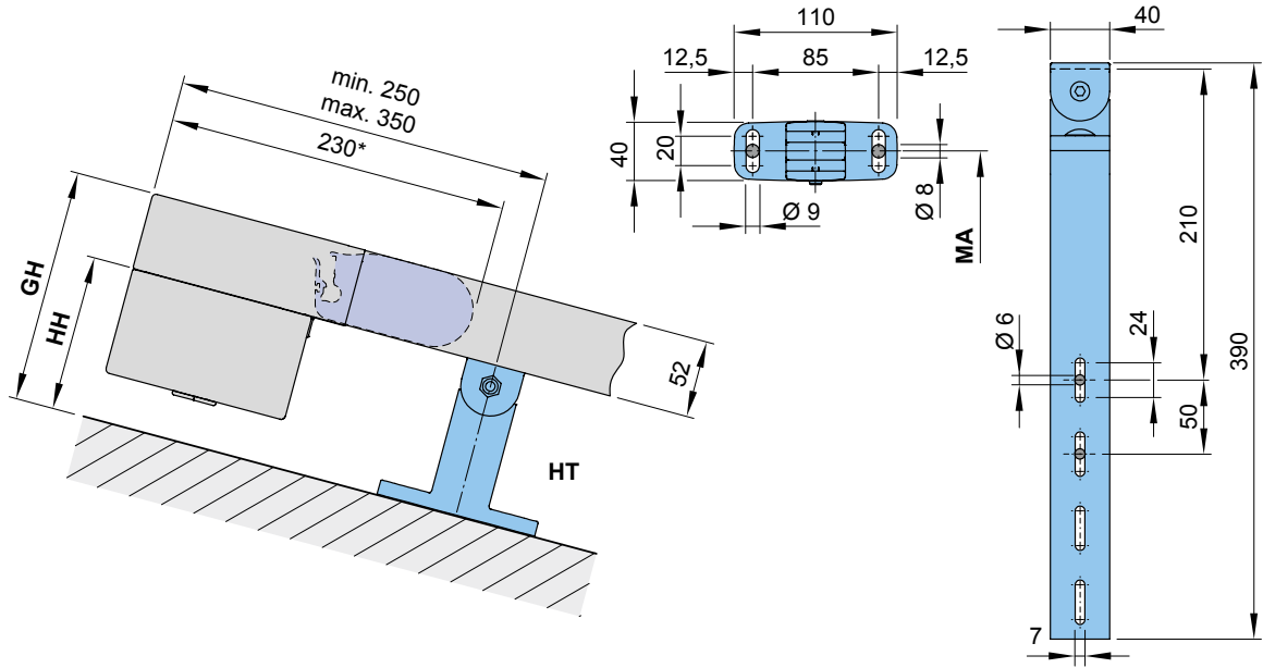
Fixture type 21,22
