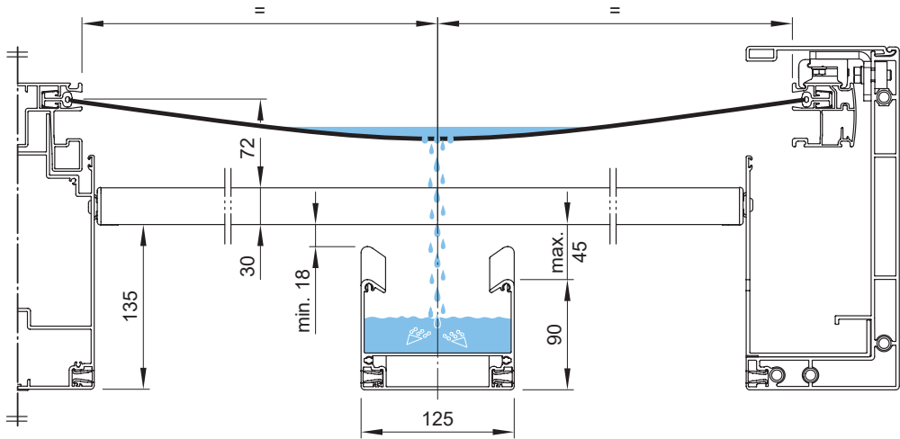
Dimension overview of the drainage gutter
